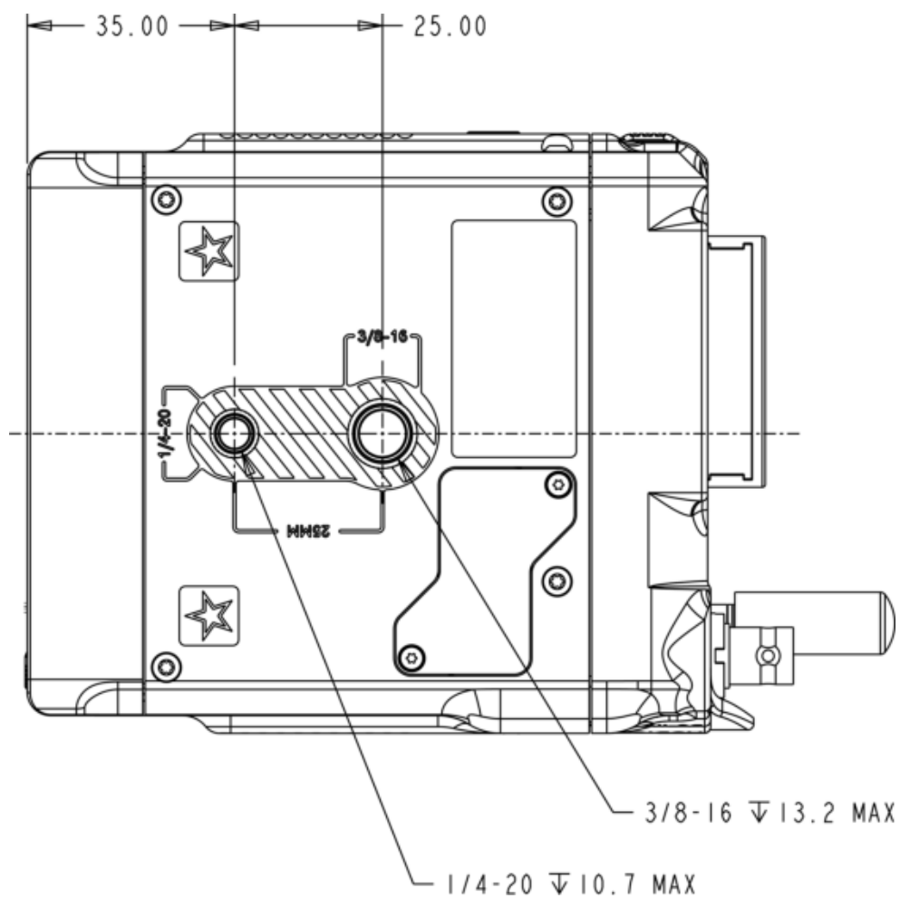
Figure: Camera Bottom View , Z Mount
