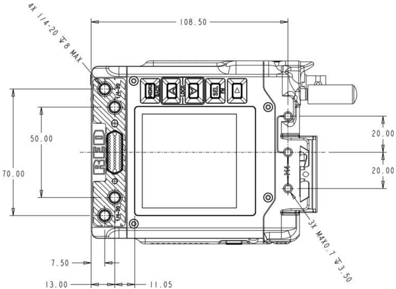
Figure: Camera Top View , Z Mount
