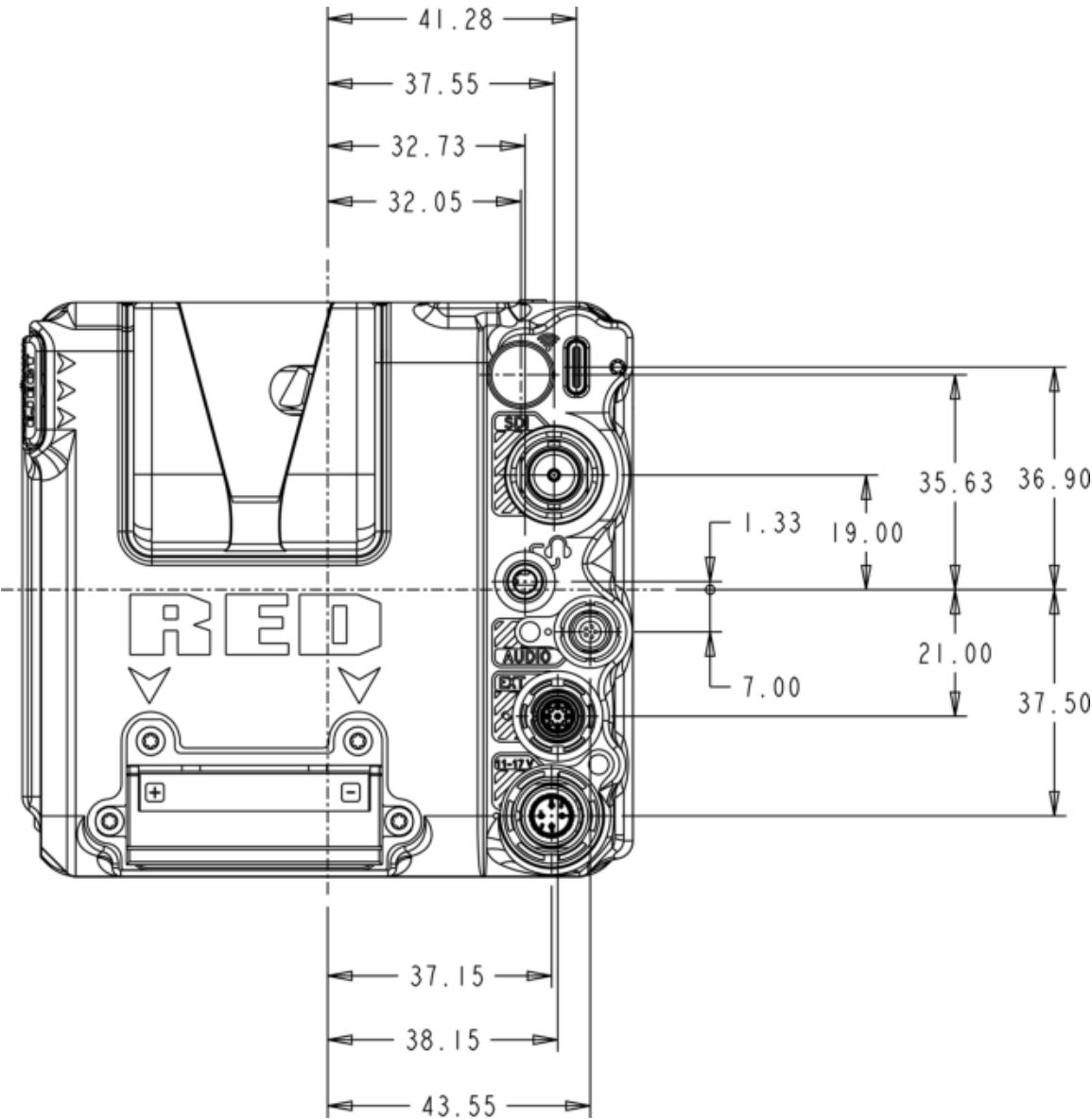
Figure: Camera Back View, Z Mount
