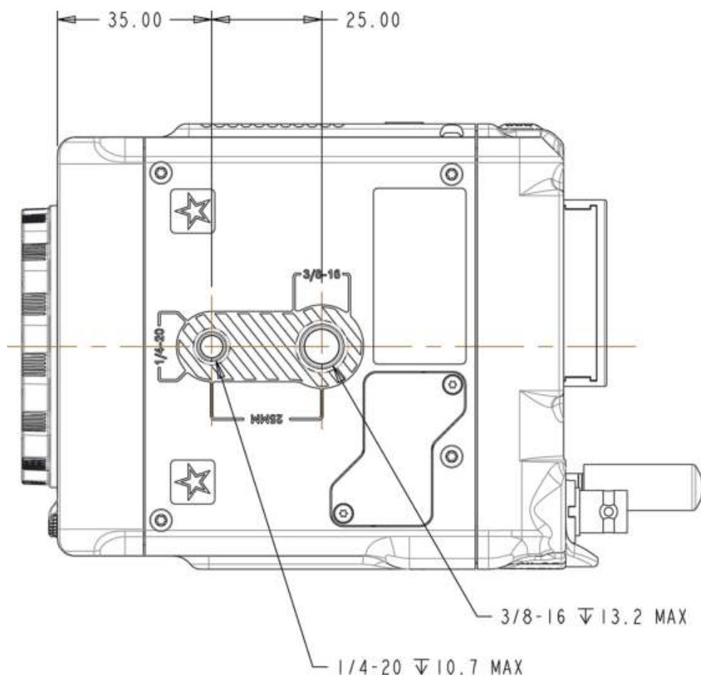
Figure: Camera Bottom View , RF
