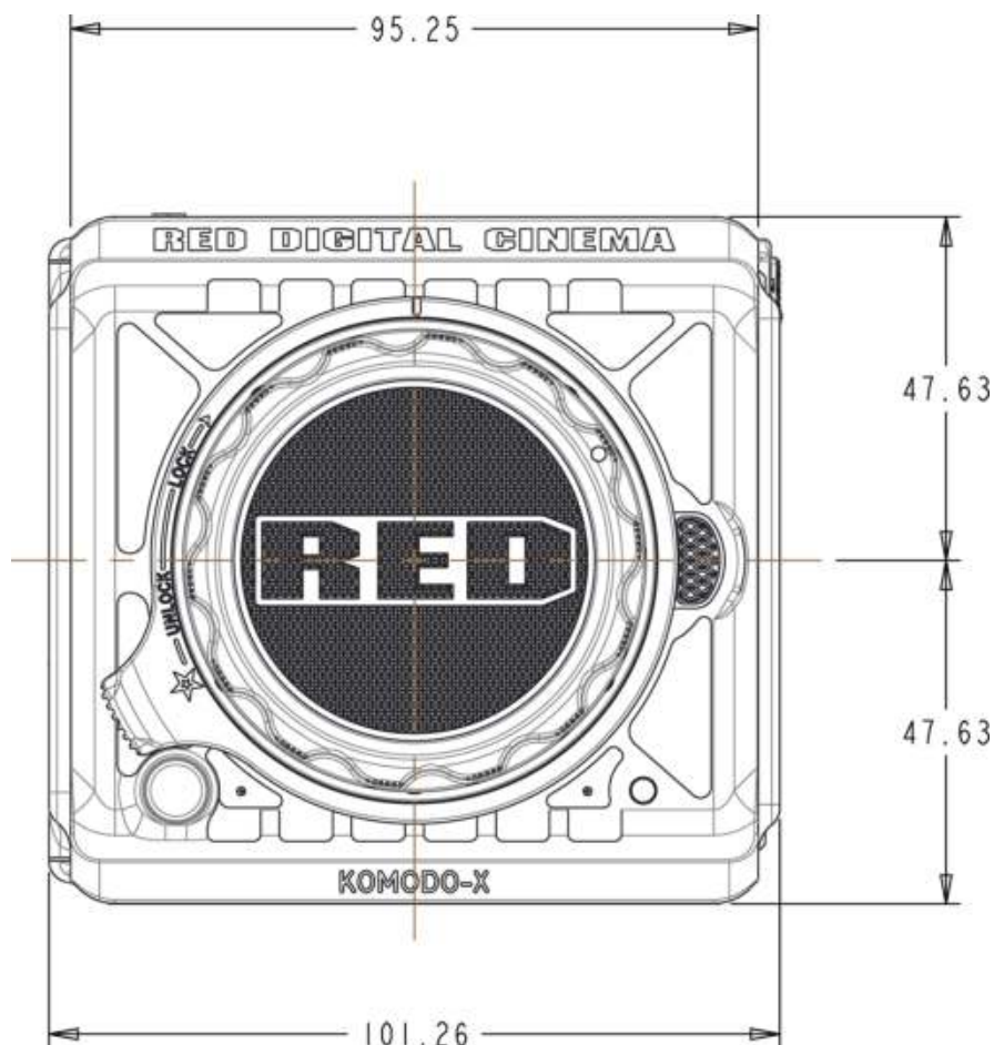
Figure: Camera Front View, RF
