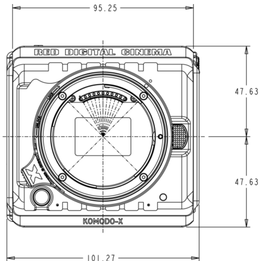
Figure: Camera Front View, Z Mount
