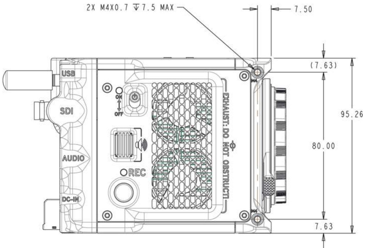
Figure: Camera Right Side View, RF
