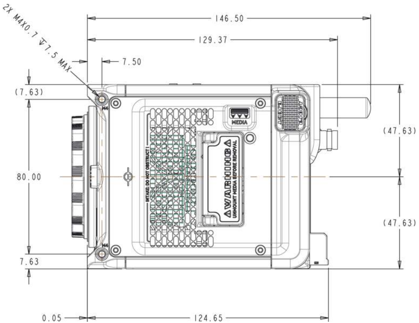
Figure: Camera Left Side View, RF
