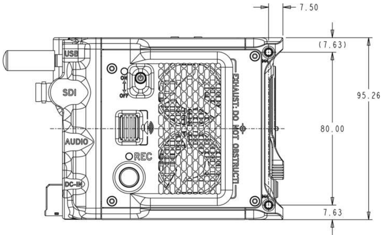
Figure: Camera Right Side View, Z Mount
