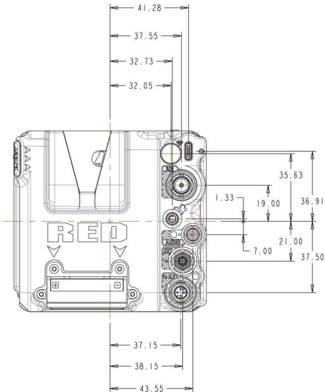
Figure: Camera Back View, RF
