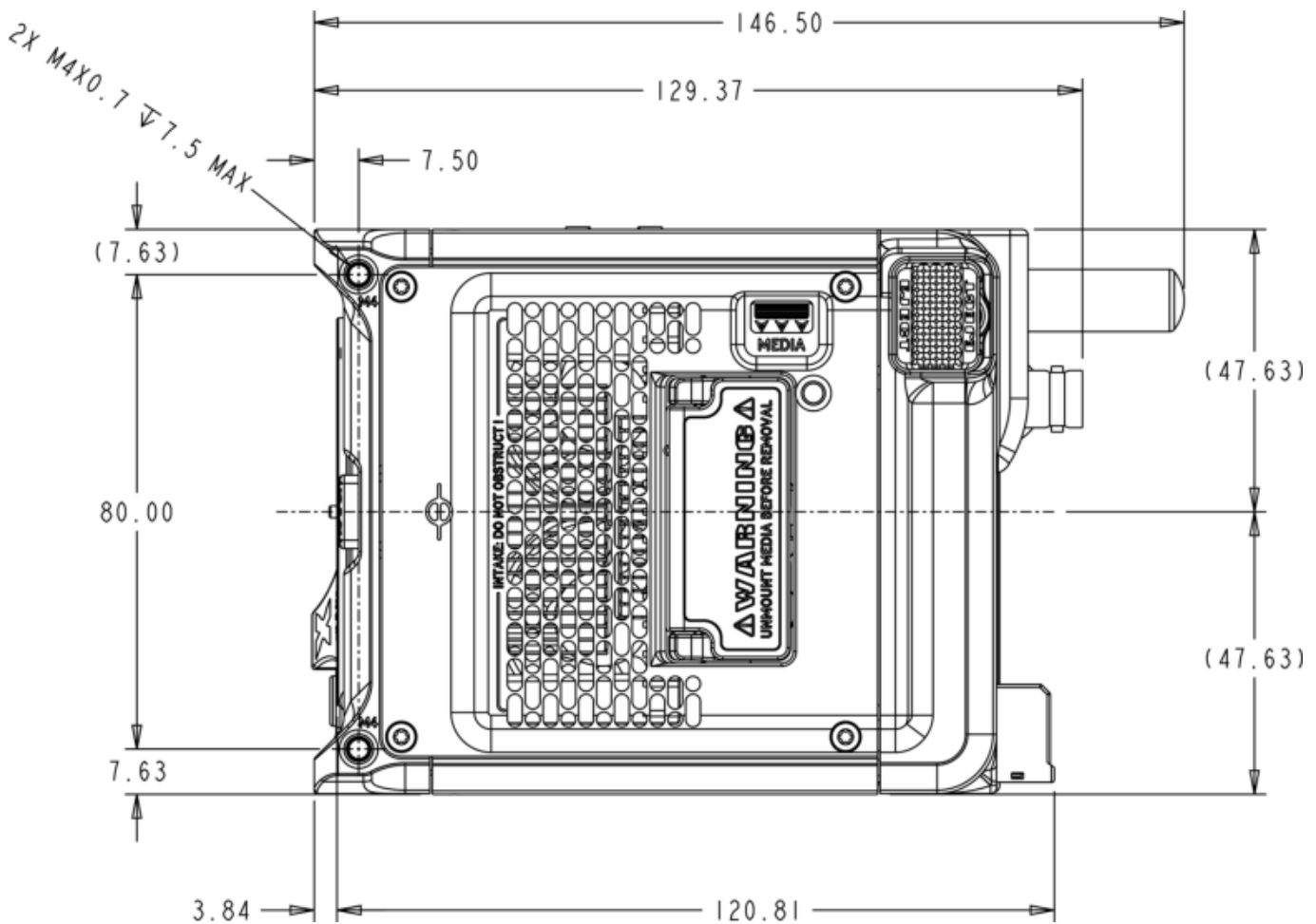
Figure: Camera Left Side View, Z Mount
