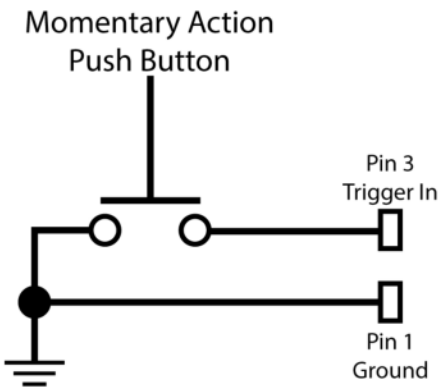
Figure: Contact Closure Style Trigger Button Circuit Diagram (24V RS)
