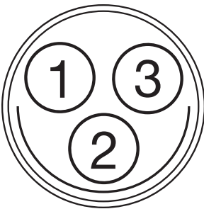
Figure: START/STOP Connector (Looking at the Connector)
