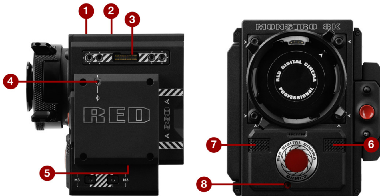
Figure: DSMC2 MONSTRO Ports and Features
