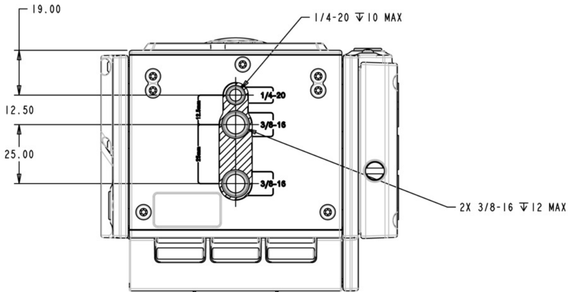
Figure: Camera Bottom View
