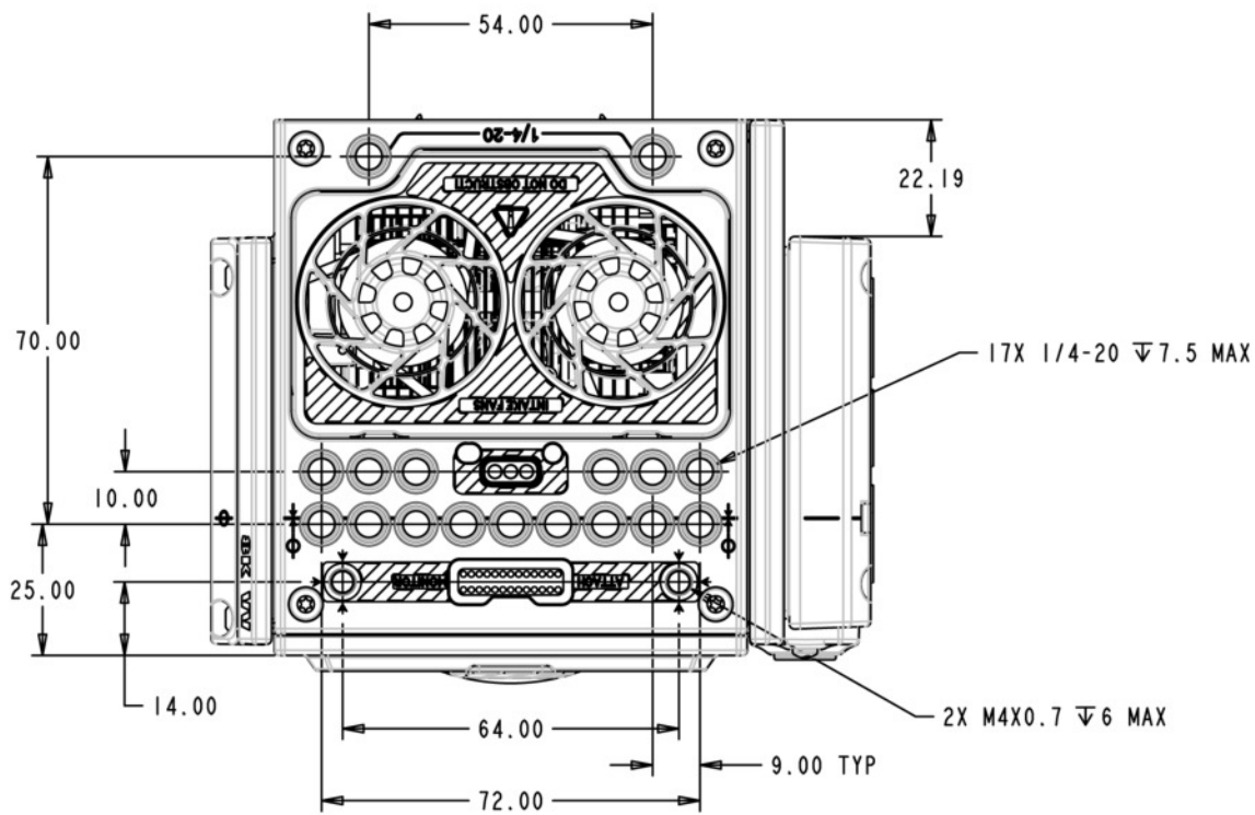
Figure: Camera Top View
