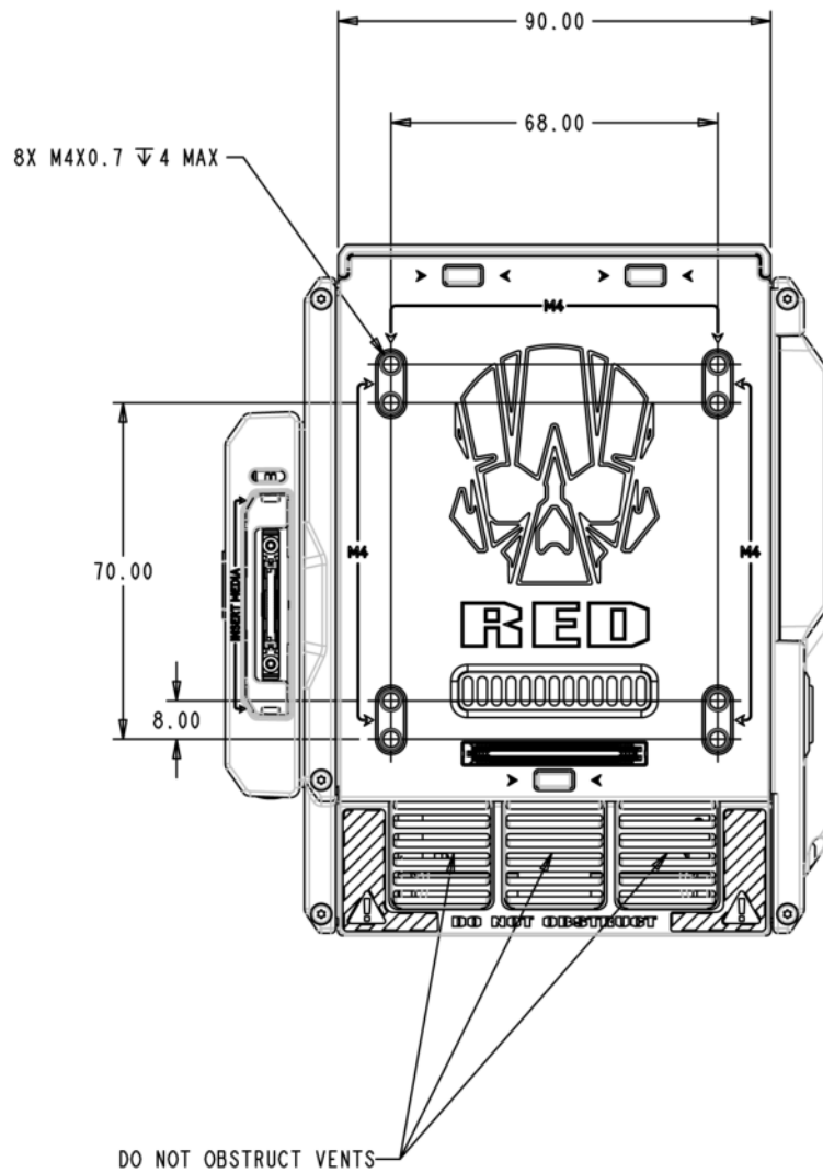
Figure: Camera Back View
